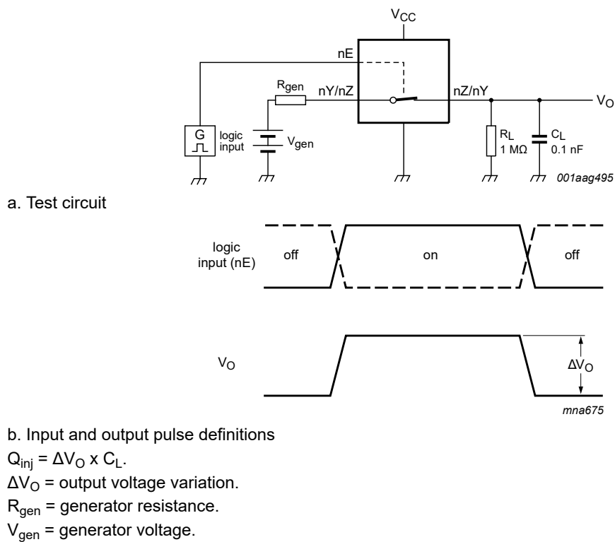
Fig. 19. Test circuit for measuring charge injection
