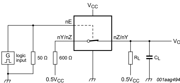
Fig. 17. Test circuit for measuring crosstalk voltage (between digital inputs and switch)
