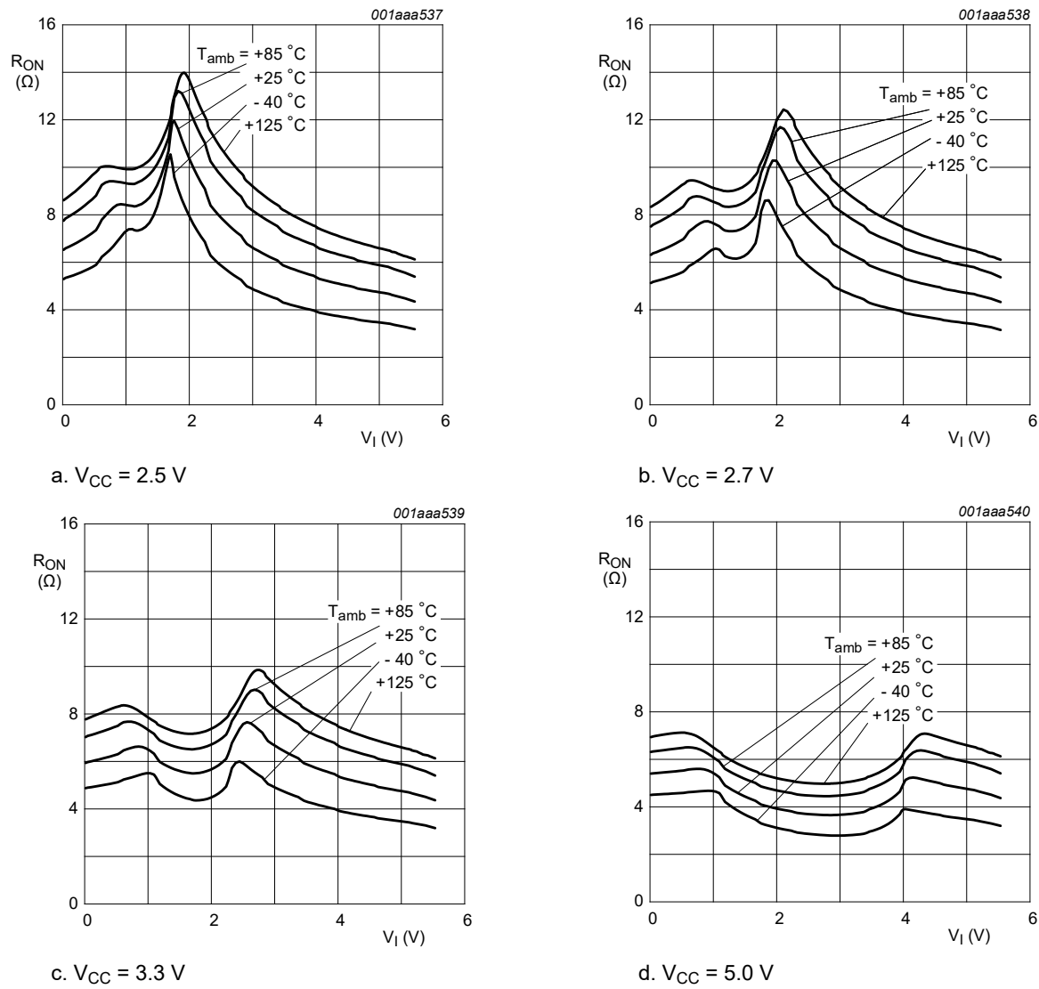
Fig. 10. ON resistance as a function of input voltage at various supply voltages
